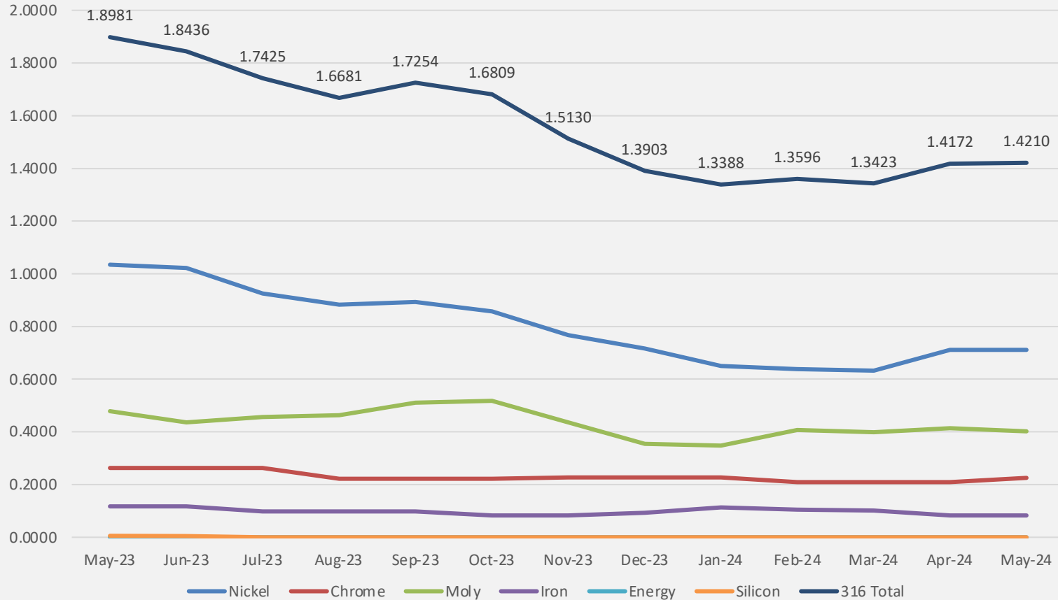
316/316L Surcharges
